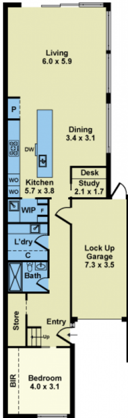
GROUND FLOOR
