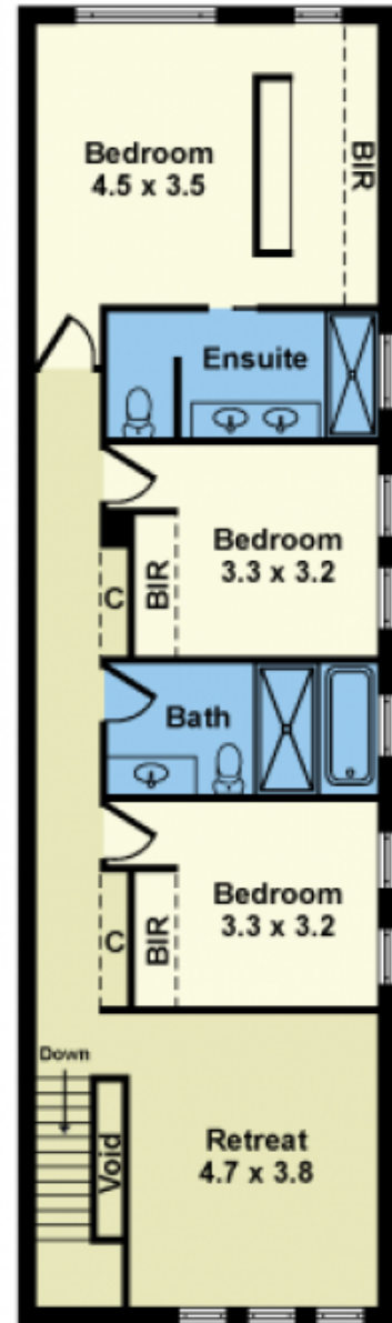
FIRST FLOOR
