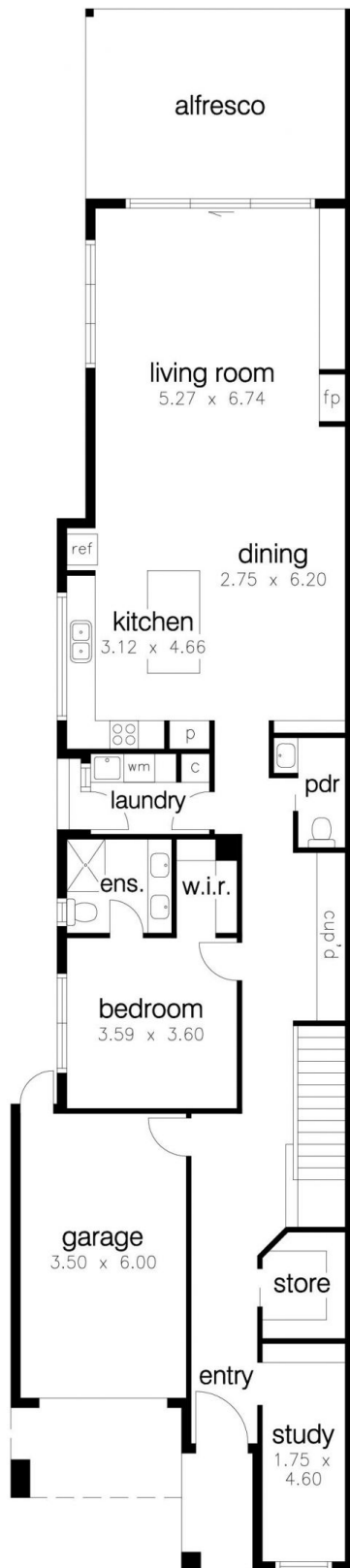
Ground Floor
